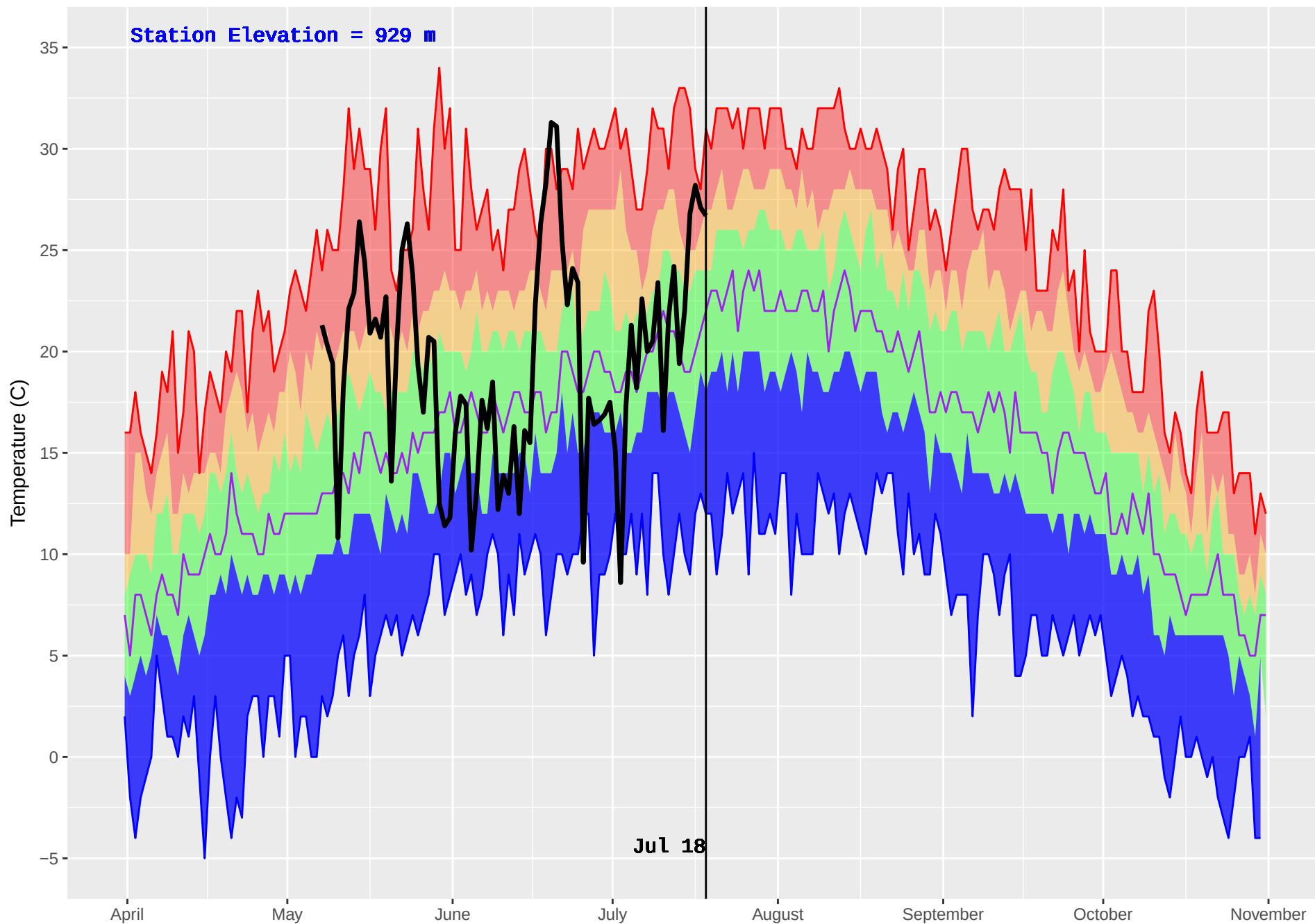
RISKE CREEK (210) : Historical (1980–2016) and Current (2018) Daily Temperature
