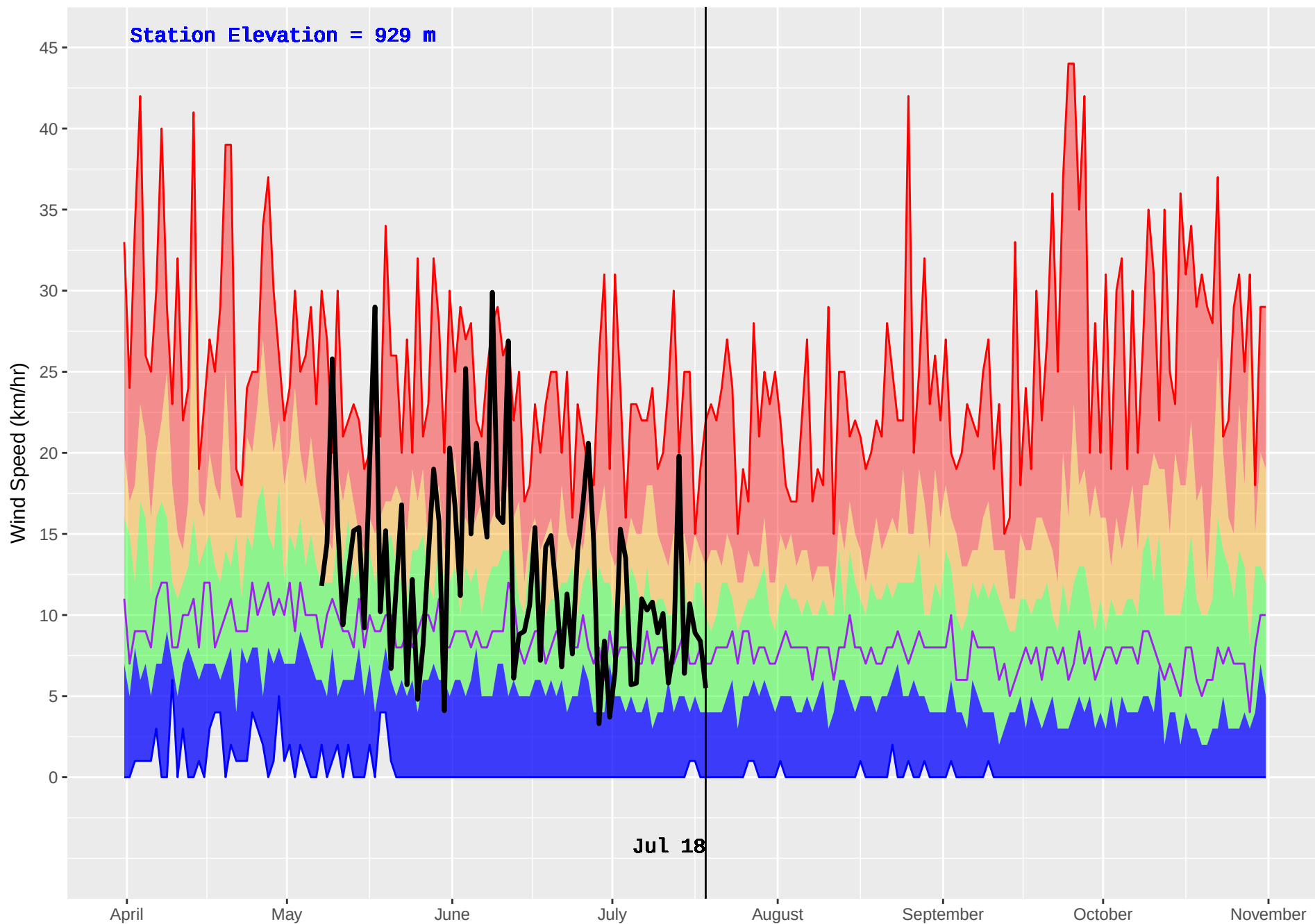
RISKE CREEK (210) : Historical (1980–2016) and Current (2018) Daily Wind Speed
