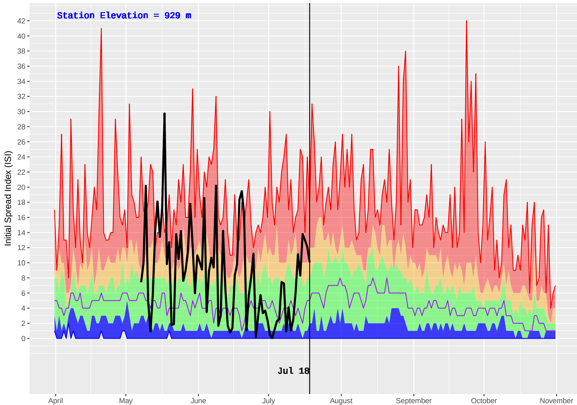
RISKE CREEK (210) : Historical (1980–2016) and Current (2018) Daily Initial Spread Index (ISI)
